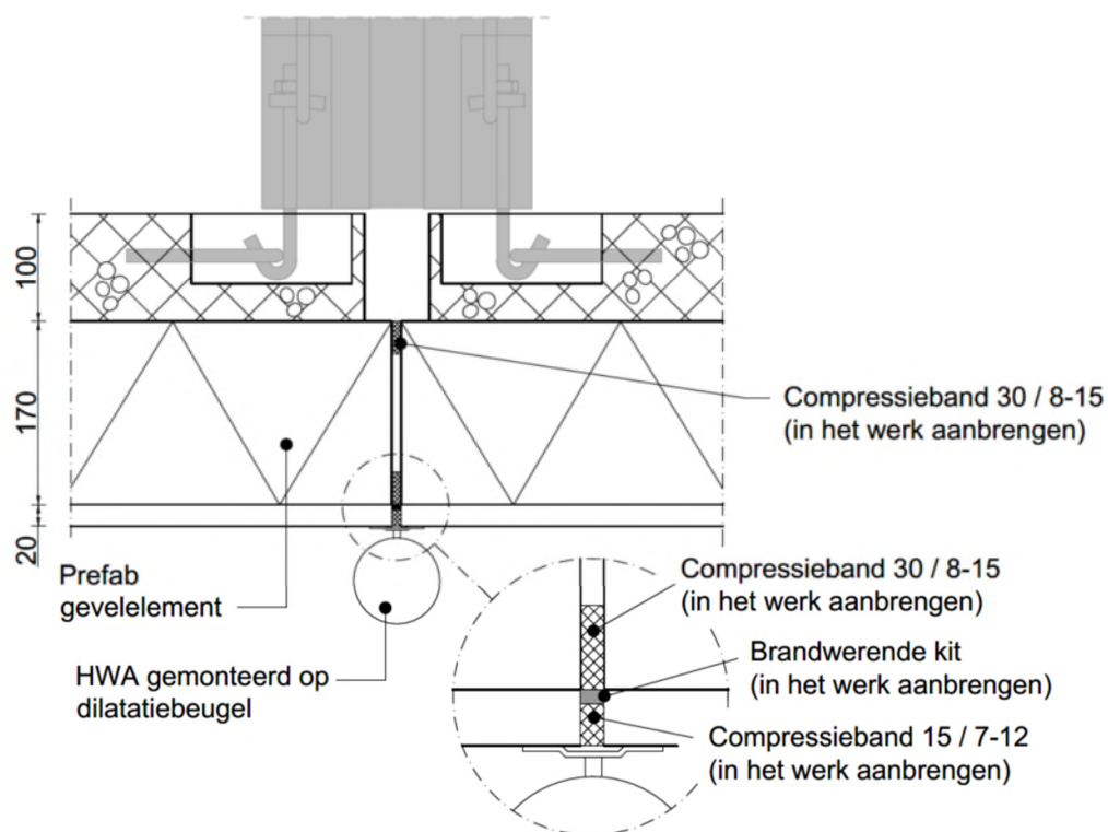
Figuur 11 – Detail wandverbindingen
